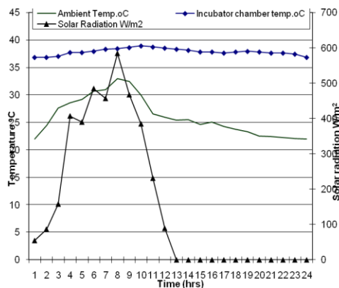
Fig. 4: Ambient and incubator temperature profiles with time.
