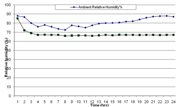
Fig. 5: Ambient and incubator relative humidity with time.
