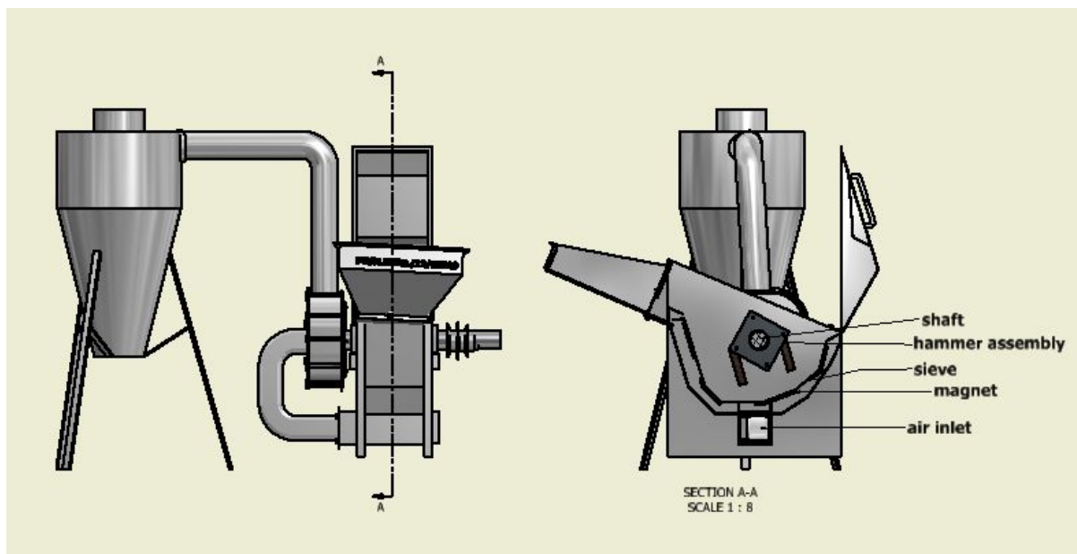
Fig.1 Cross section A-A of the Magnetic Sieve Grinding Machine
