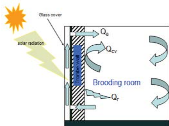
Figure 2: Heat transfer mechanism within a typical Trombe wall poultry house.
