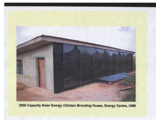
Figure 1: 2000 capacity Trombe wall day-old poultry brooding house.
