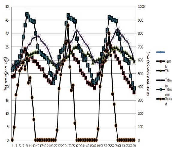
Figure 6: Temperature and solar radion profiles vs time (day).
