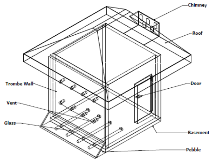
Figure 1 Three dimensional sketch of Trombe wall solar chick brooder
