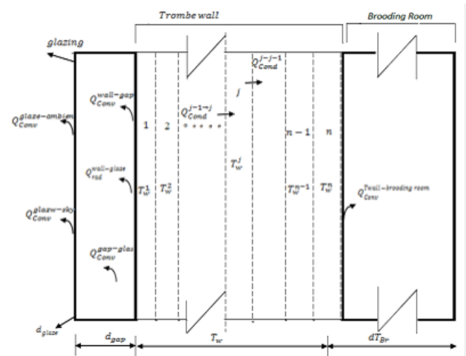
Figure 3 Discretization of the Trombe wall showing thermal energy transfers
